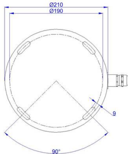
MOUNTING HOLES
